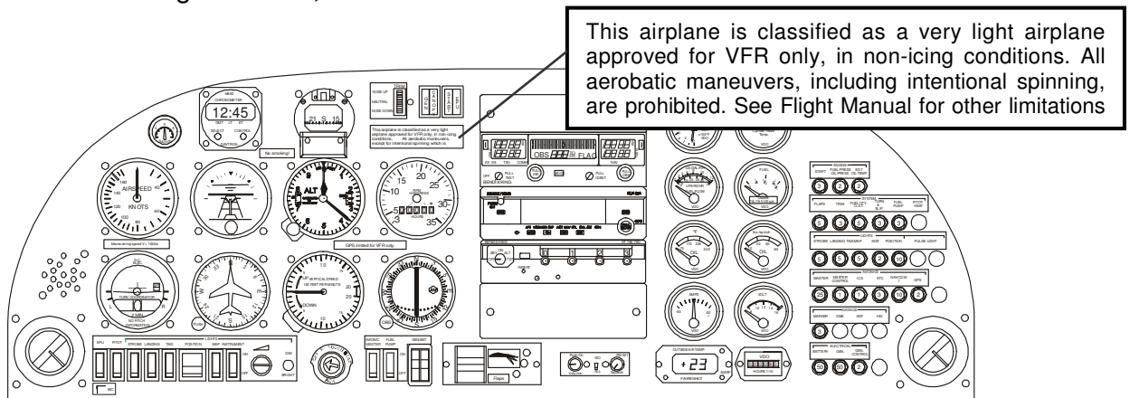
Figure 1 – VLA Label placement on the instrument panel
